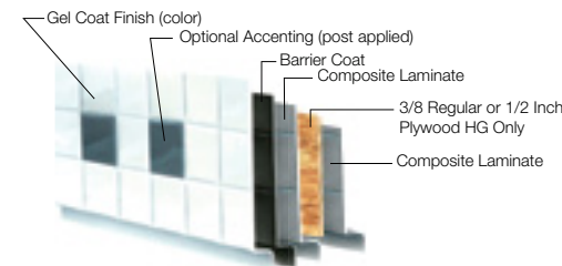
Composite Floor Structure
