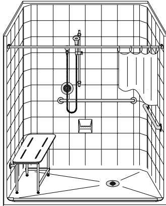
PERSPECTIVE VIEW - N.T.S. MODEL SHOWN HERE AS: LEFT SEAT LEFT PLUMBING RIGHT DRAIN
