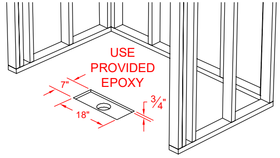
FOR MODELS ENDING IN A75FT*.V3, INSTALLATION REQUIRES A 7" x 18" x \frac{3}{4} " CUT-OUT.
